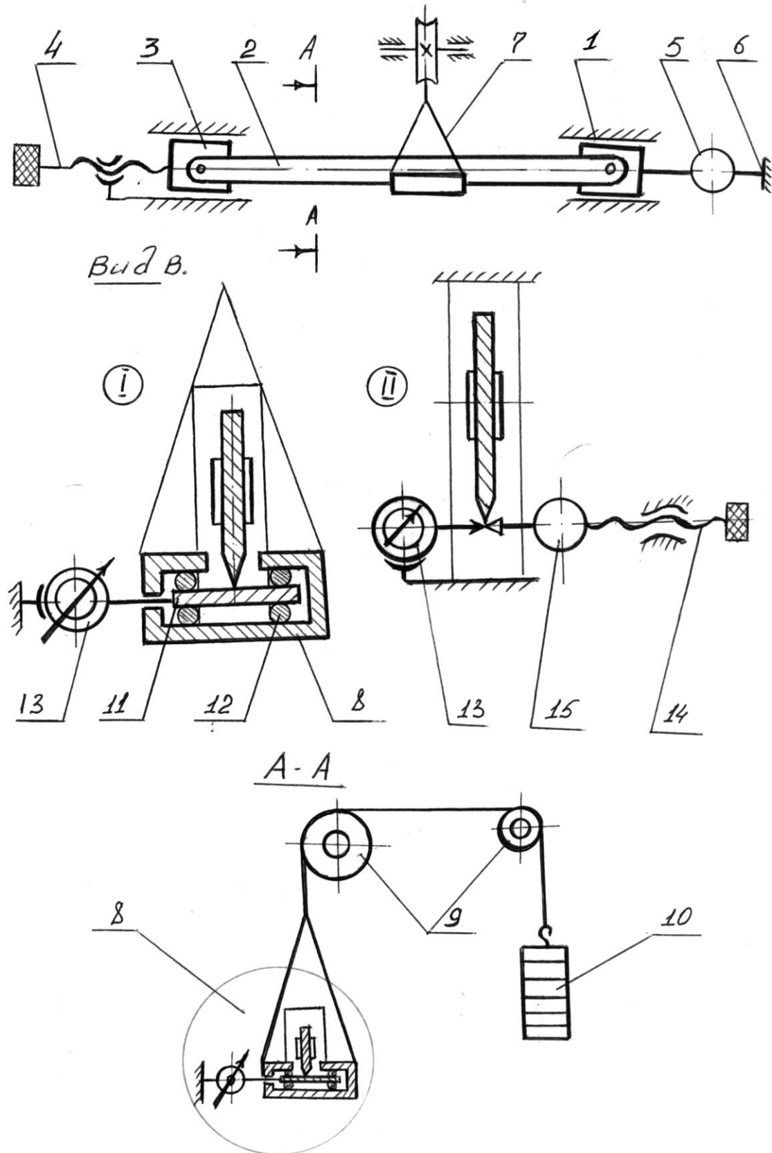
Fig. 1. Schematic diagram of the experimental installation
