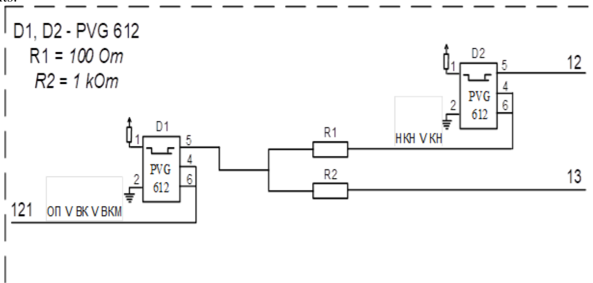
Figure.1 The NPM-69 block. uses an electrical circuit for connecting power to the circuit of automatic push-button relays (ACN) and the relay circuit of the switch control (PU, MU) of the PVG-612 optorele block..
