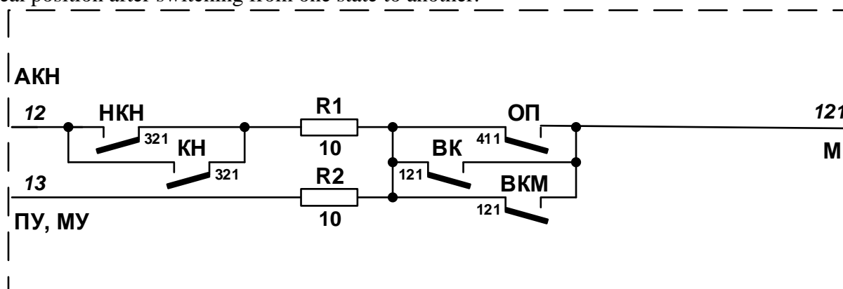
Figure.1 Circuit diagram of automatic push-button relays (ACN) and switch control relay circuits (PU, MU) in the NPM-69 block.
