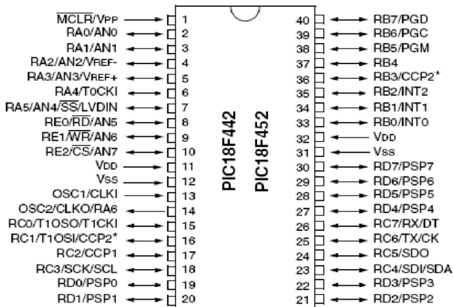
1.2- picture. PIC 18f452 microcontroller
